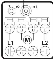
Figure 1. Wiring Diagram Figura 1. Diagrama eléctrico Figure 1. Diagramme de câblage
